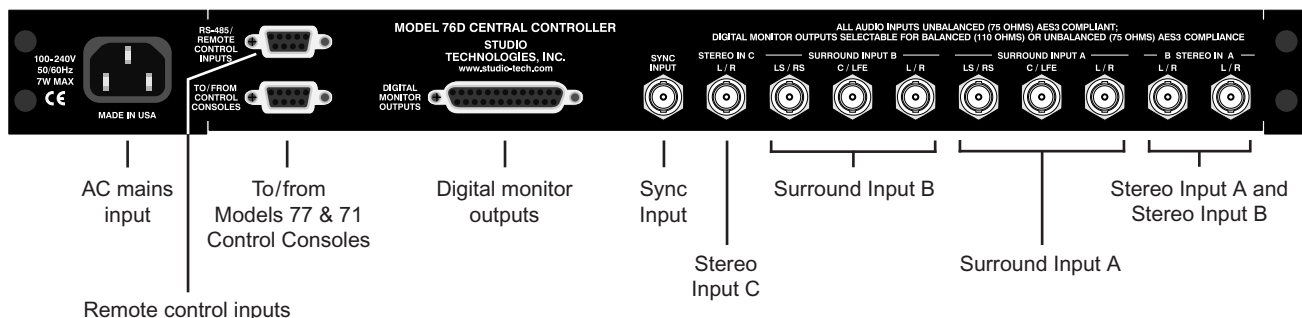
Figure 2. Model 76D Central Controller Back Panel
